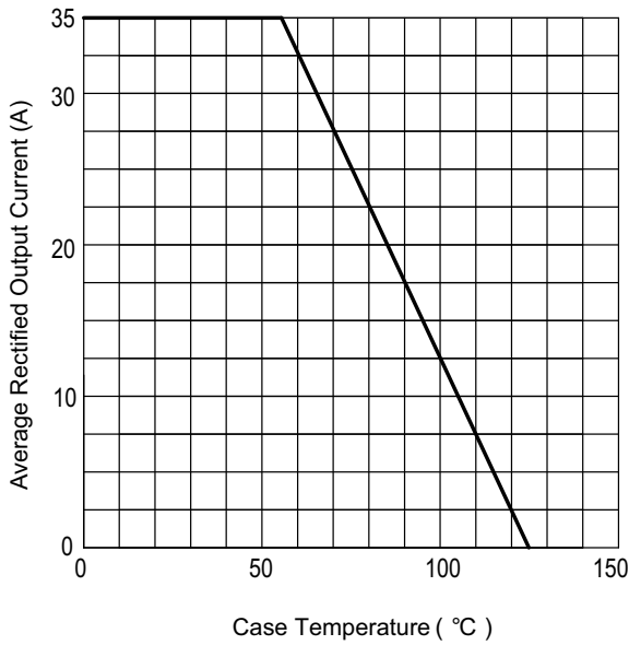
FIG1:Io-Tc Curve
